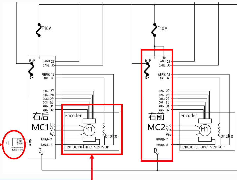
Driving motor assembly Diagram / 行走电机总成图纸
