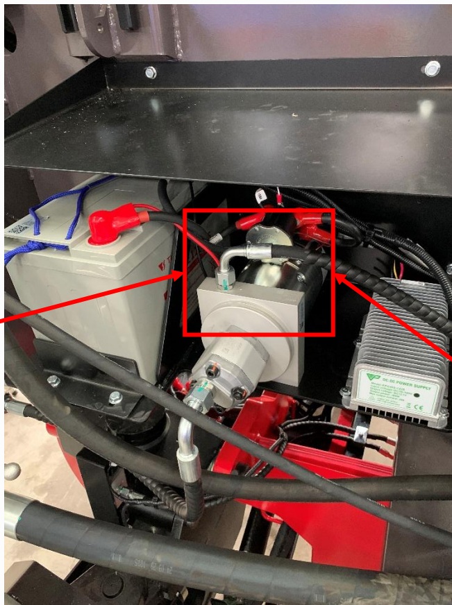
Emergency pump motor Location / 应急泵位置
