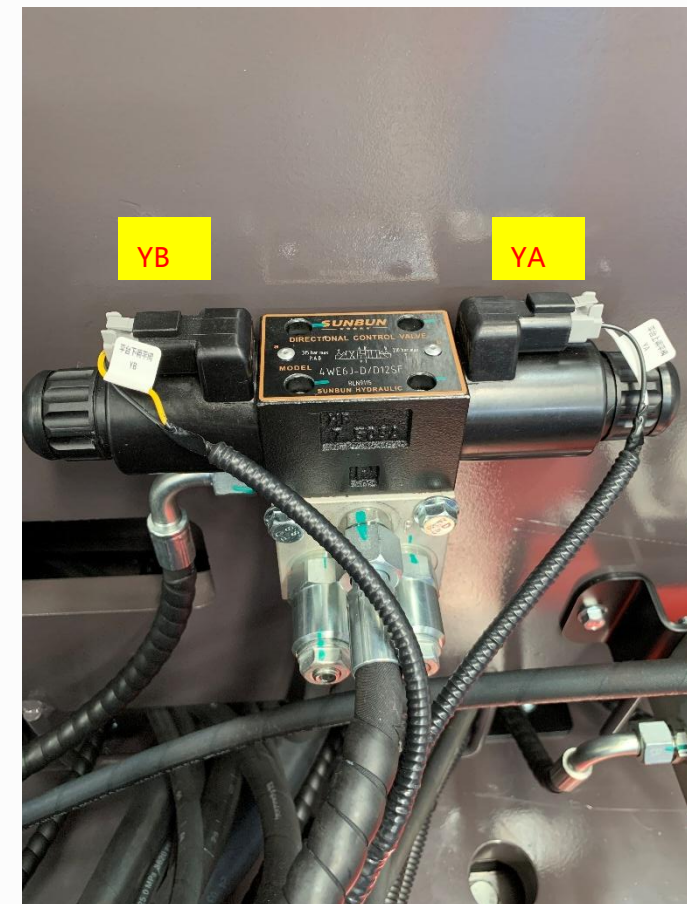
Platform tilt up & down Solenoid valve Location / 平台上下电磁阀位置
