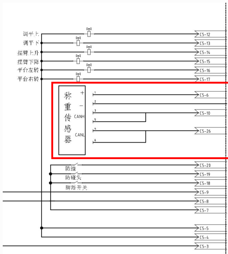
Load cell Diagram / 称重传感器图纸
