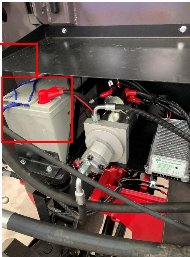
Battery location / 蓄电池位置
