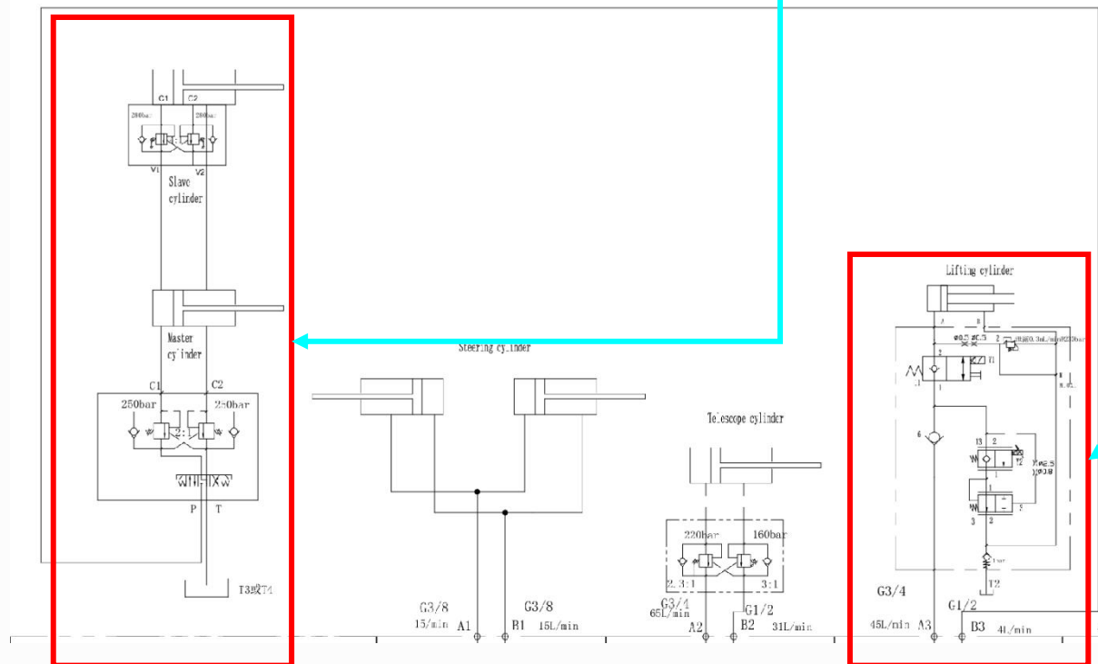
Hydraulic cylinder Diagram / 液压油缸图纸
