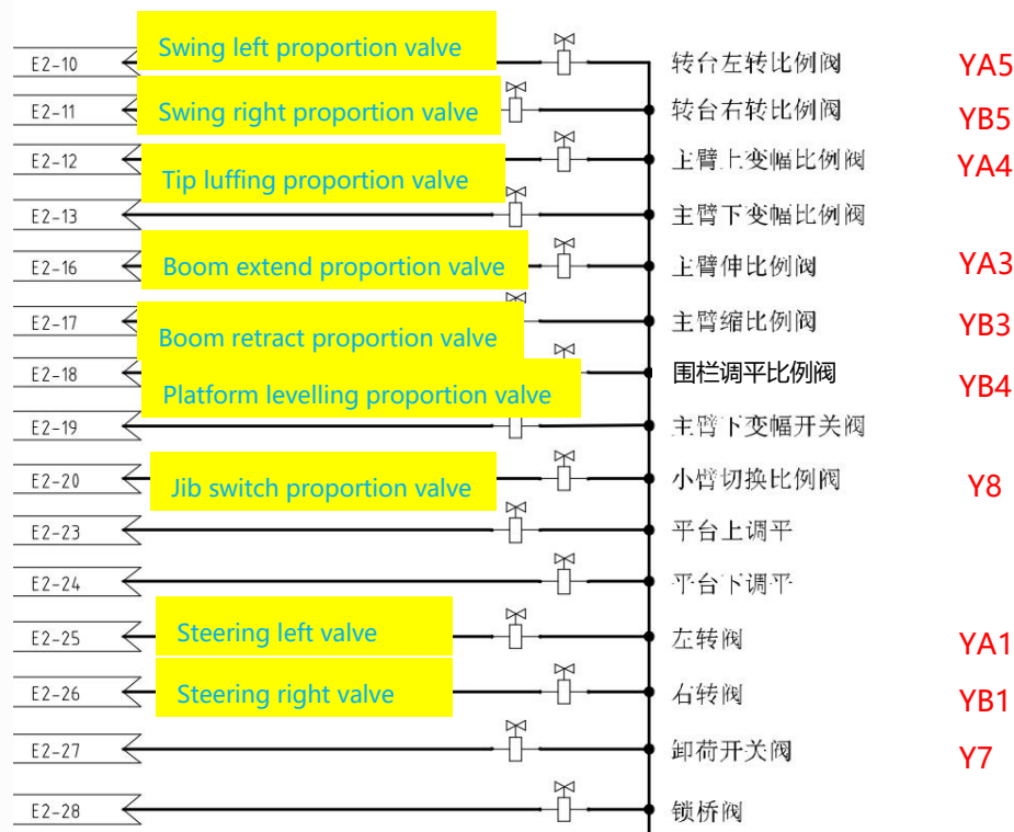
Solenoid valve Diagram / 电磁阀图纸
