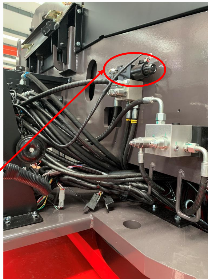
Platform tilt up & down Solenoid valve Location / 平台上下电磁阀位置
