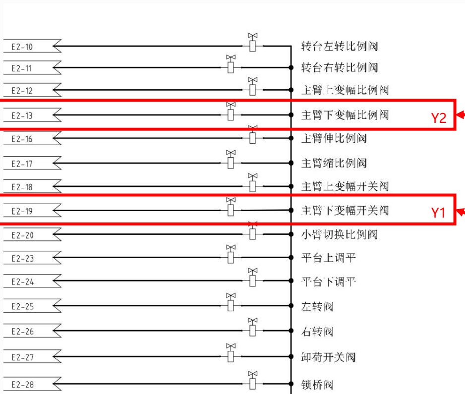
Solenoid valve Diagram / 电磁阀图纸
