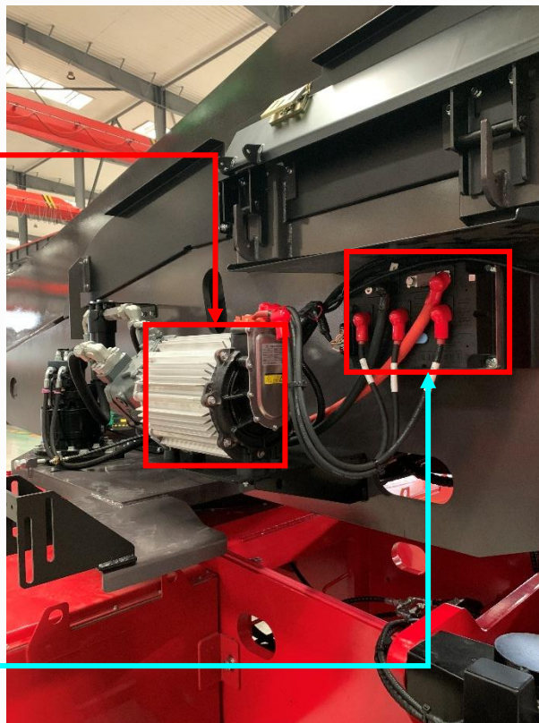
Hydraulic oil motor assembly Location / 电机马达位置图
