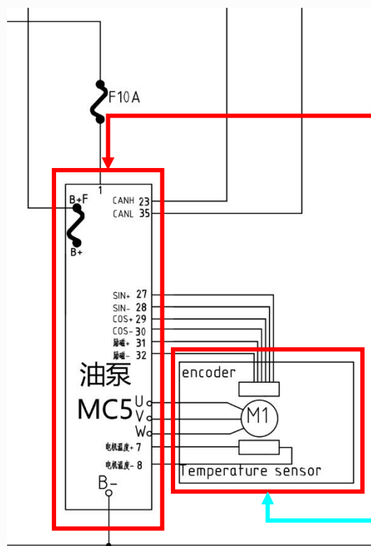
Hydraulic oil motor assembly Diagram 液压油电机马达总成图纸
